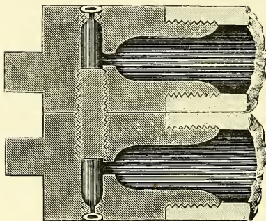
Nock's Patent Breech.
